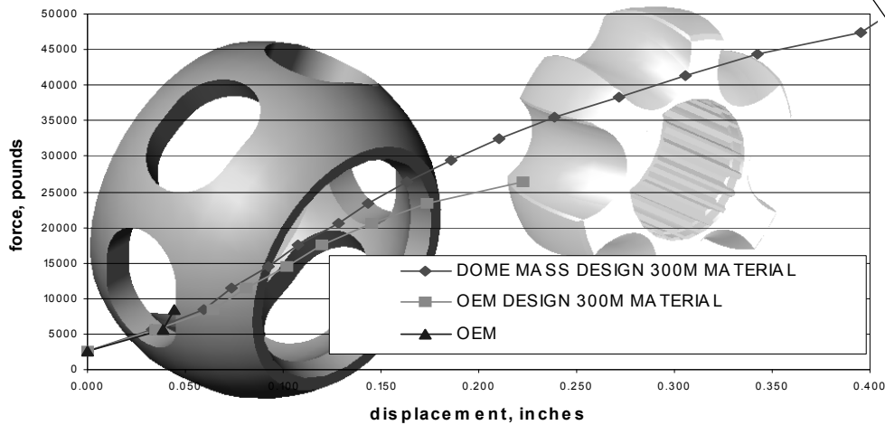
538-0 CAGE ULTIMATE STRENGTH TEST RESULTS
